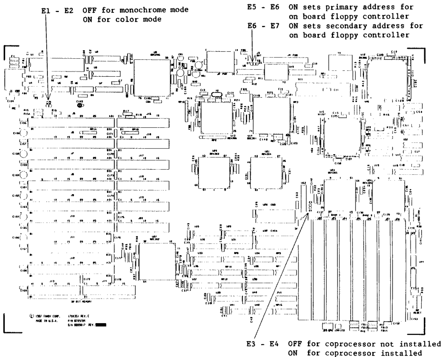
Figure 207. Tandy 4000LX Main Logic Board Revision C, C-1
