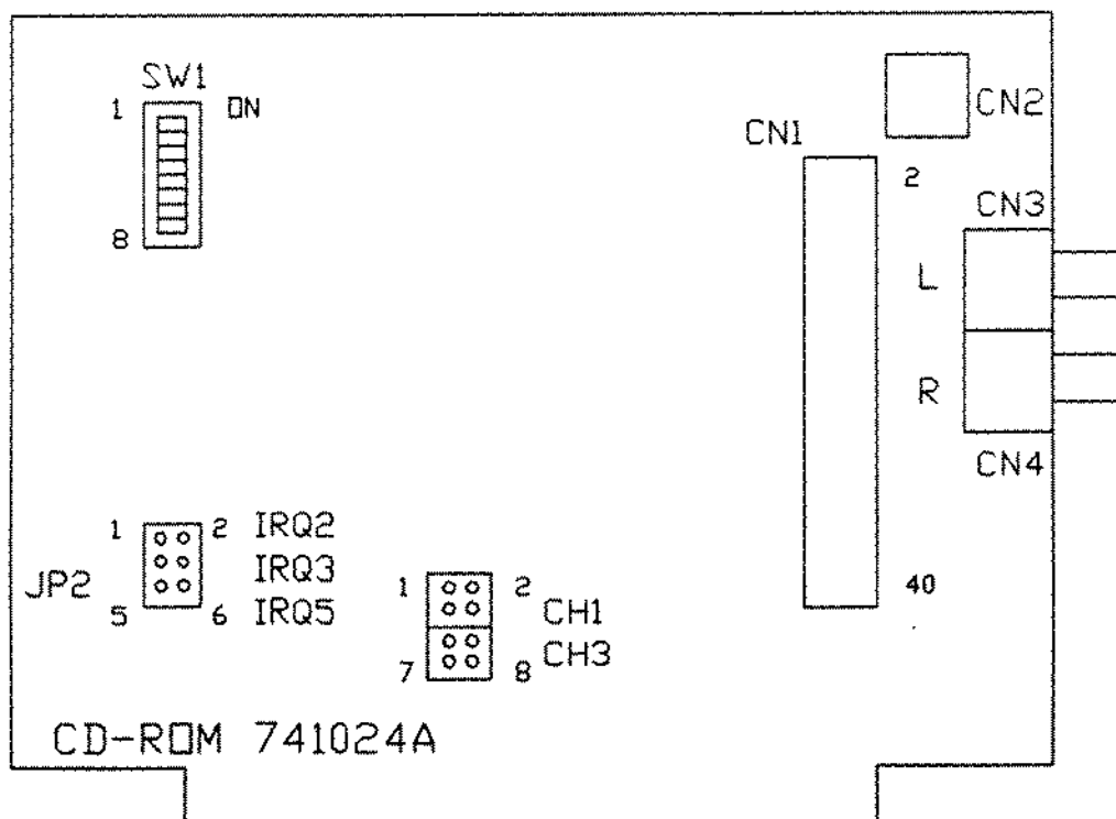
Interface Board
