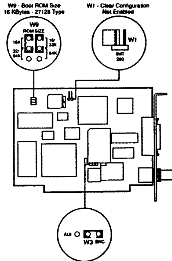
Figure 248. Tandy Ethernet Adapter Board
