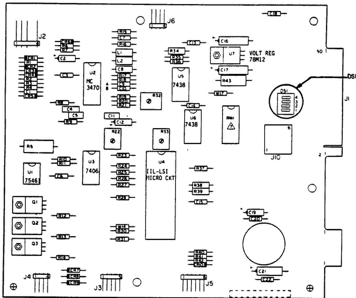
Figure 36. CDC Floppy Drive Logic Board ( LSI ).
