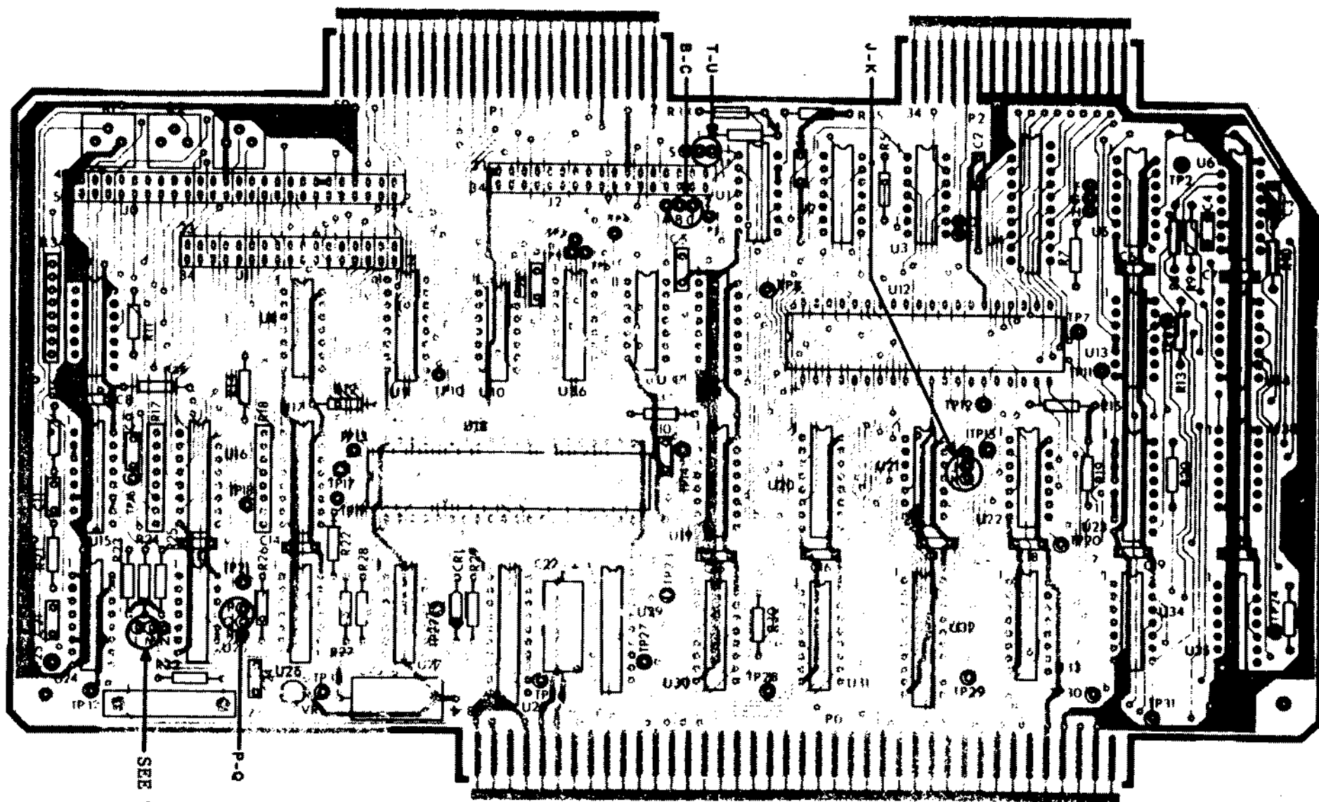
Figure 7. FDC Board ( Late Style for Model II ).
