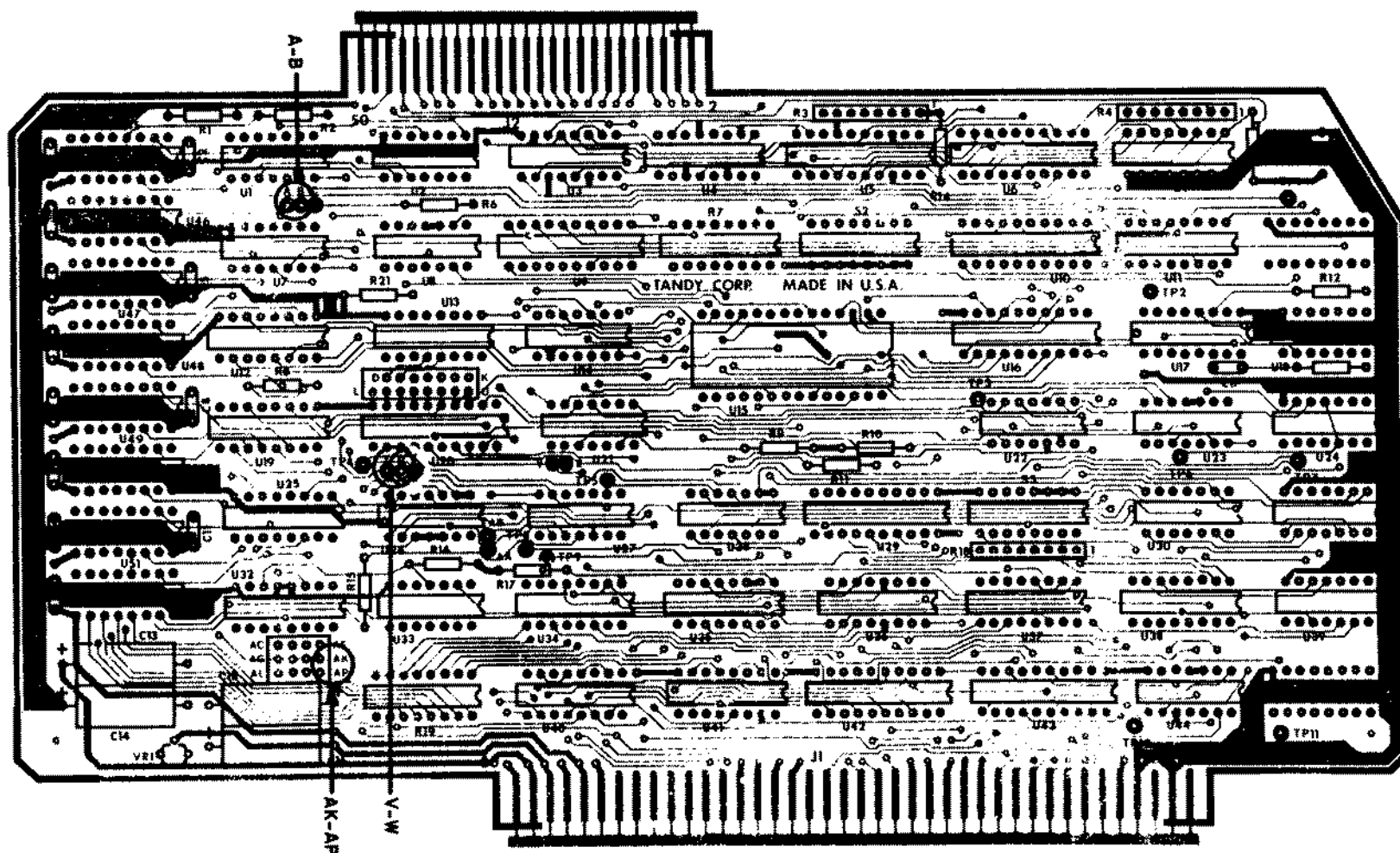
Figure 19. 8 MEG Hard Disk Interface In Model II/16/16B.
