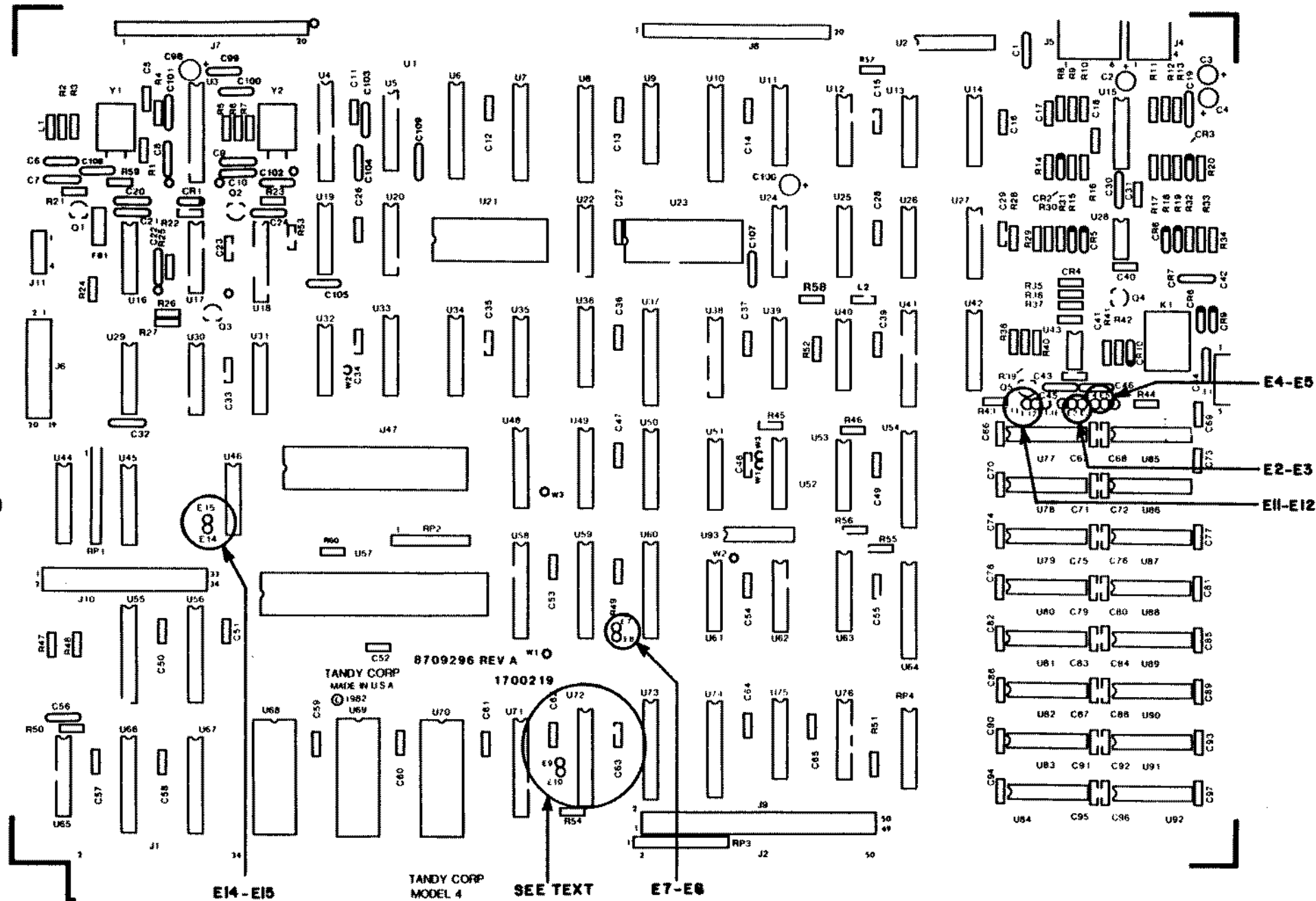
Figure 89. 64K/128K Model 4 Standard PCB.
