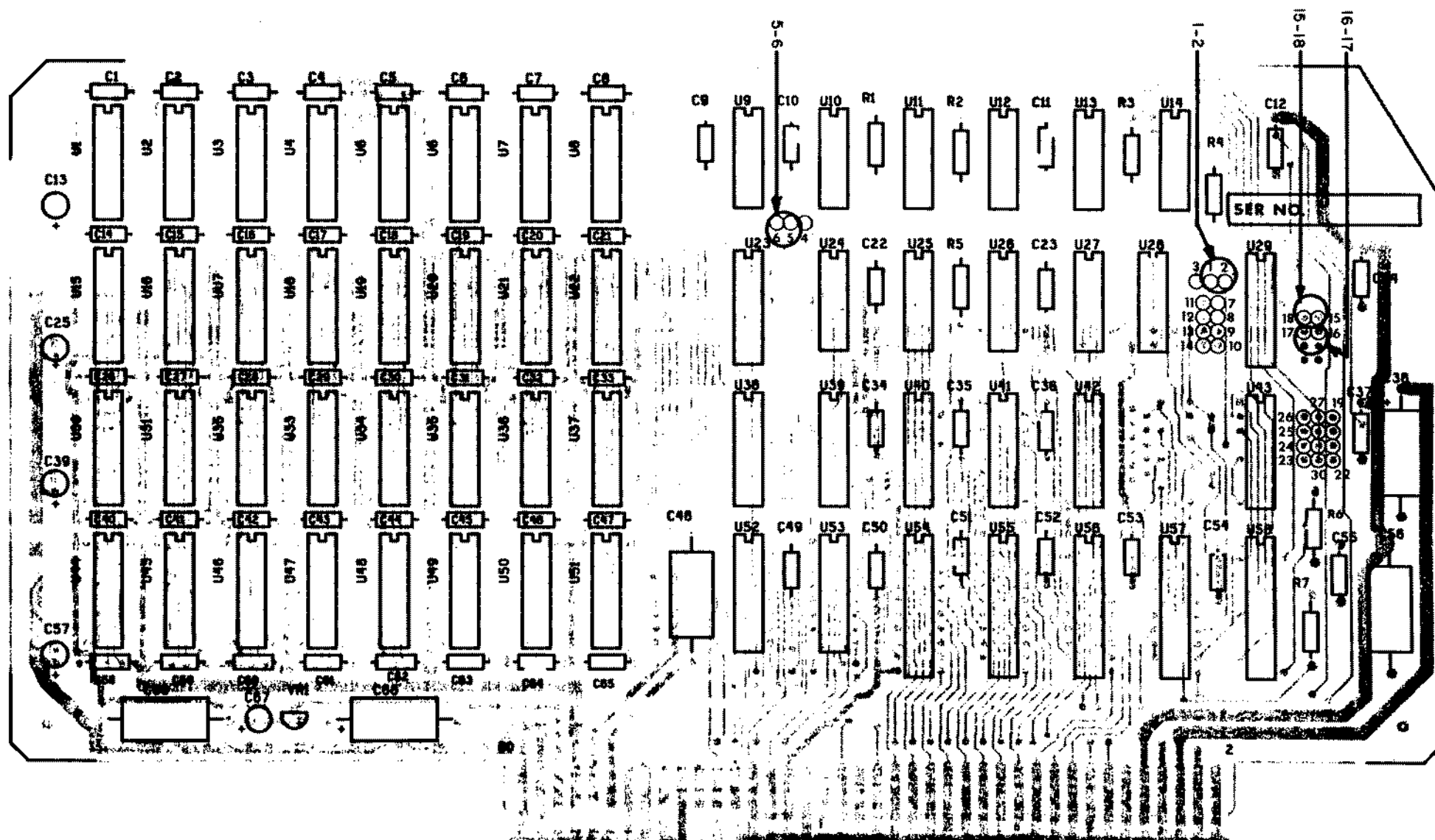
Figure 9. First 32K Memory Board.
